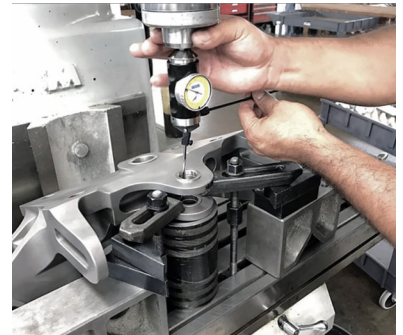
Engine Mount
